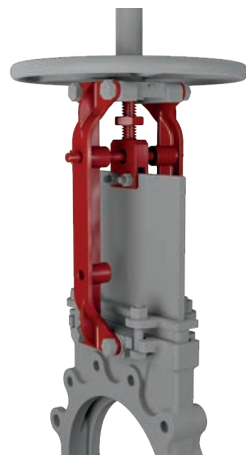
Pinned Lockout Open & Closed
